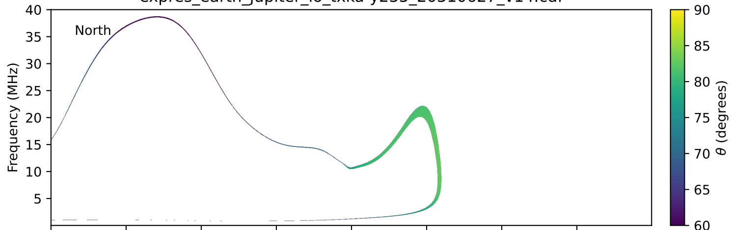
expres_earth_jupiter_io_txka-y235_20310627_v14.cdf
