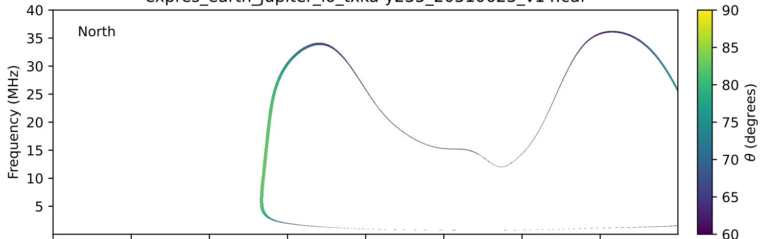
expres_earth_jupiter_io_txka-y235_20310623_v14.cdf
