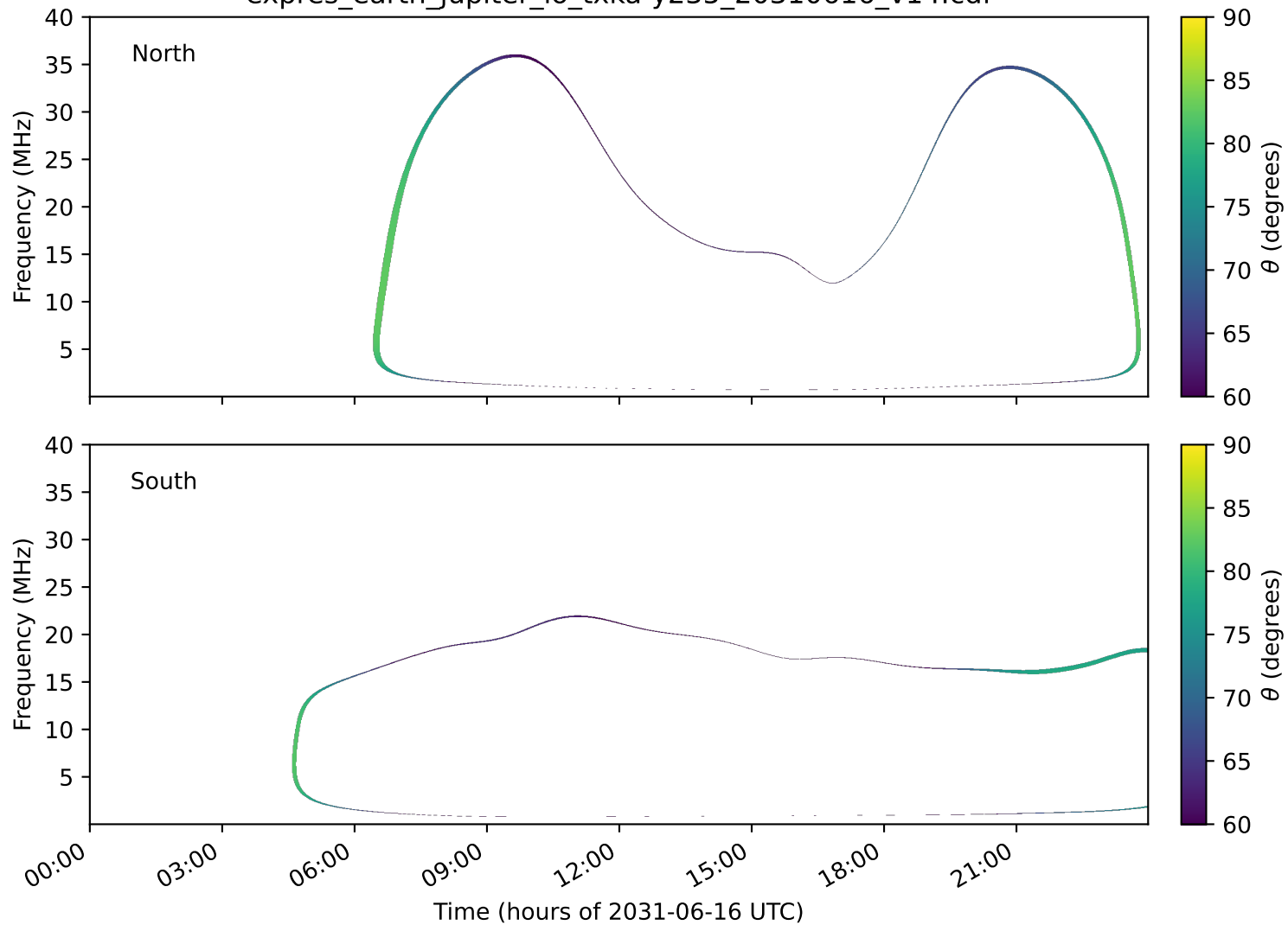
expres_earth_jupiter_io_txka-y235_20310616_v14.cdf
