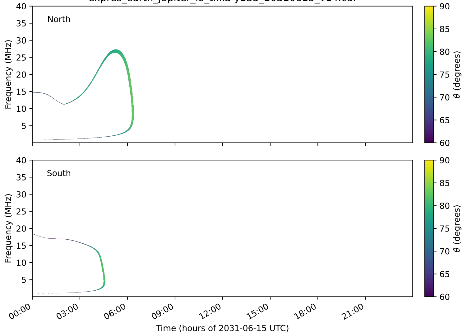
expres_earth_jupiter_io_txka-y235_20310615_v14.cdf
