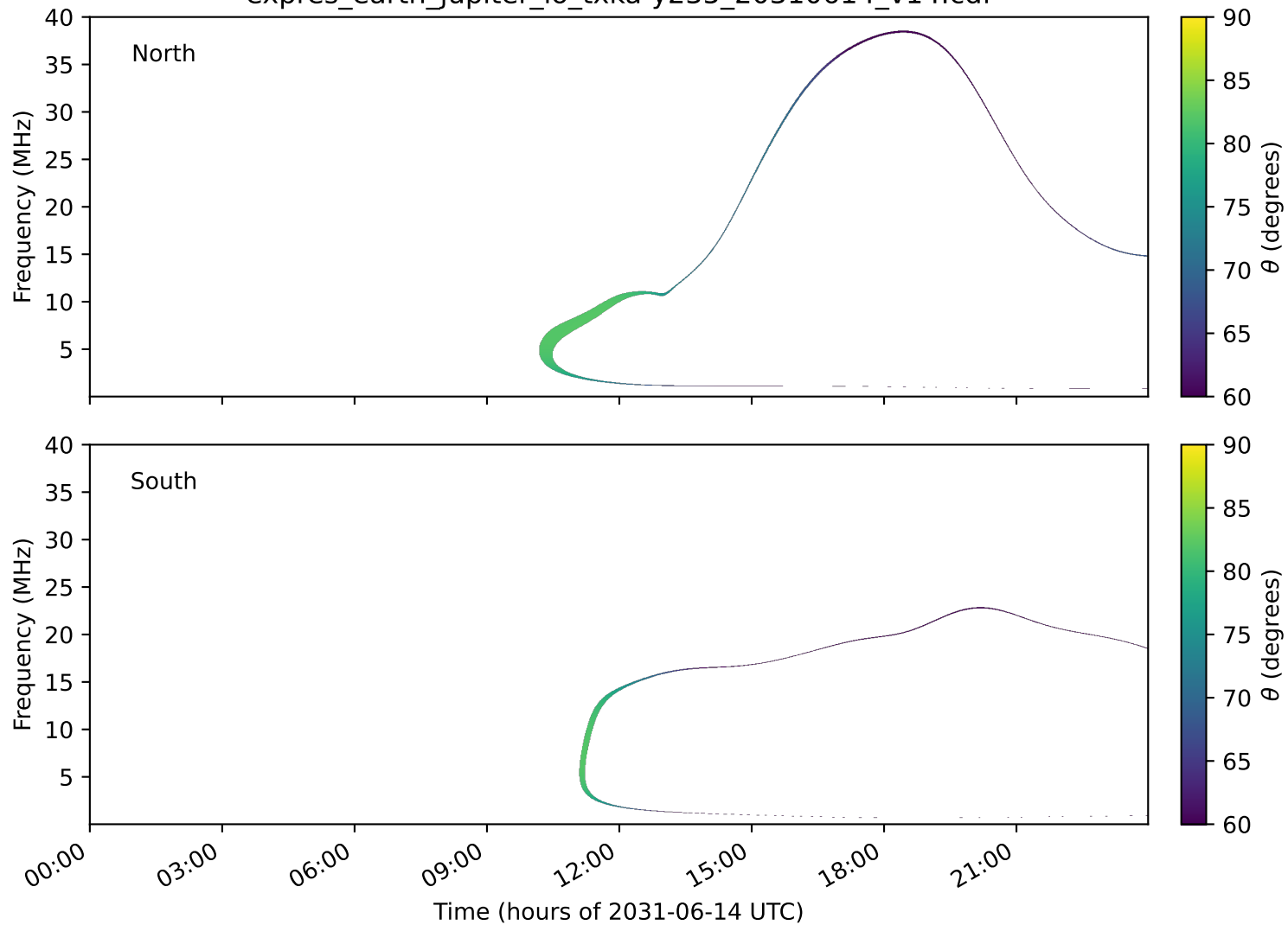
expres_earth_jupiter_io_txka-y235_20310614_v14.cdf
