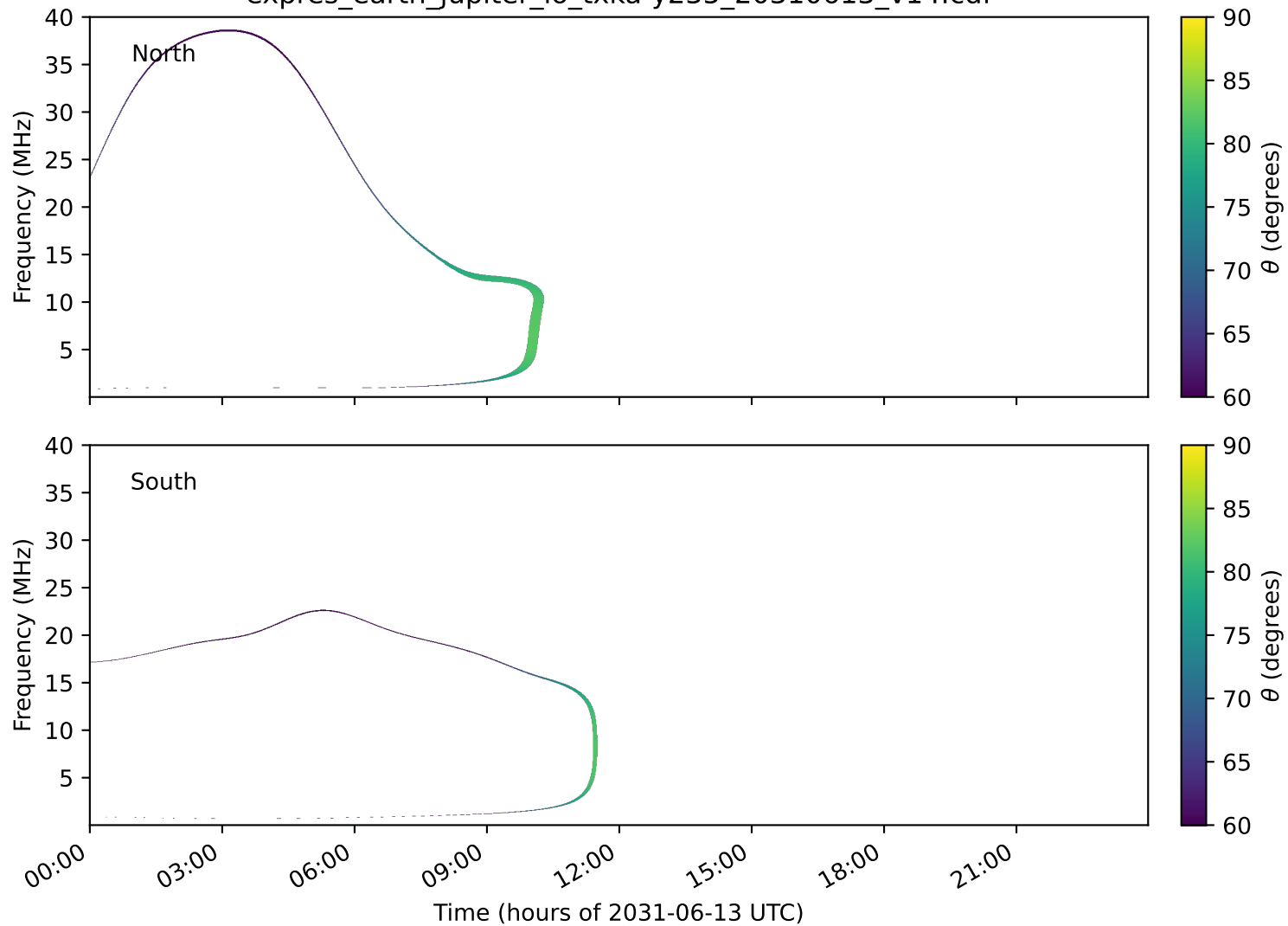
expres_earth_jupiter_io_txka-y235_20310613_v14.cdf
