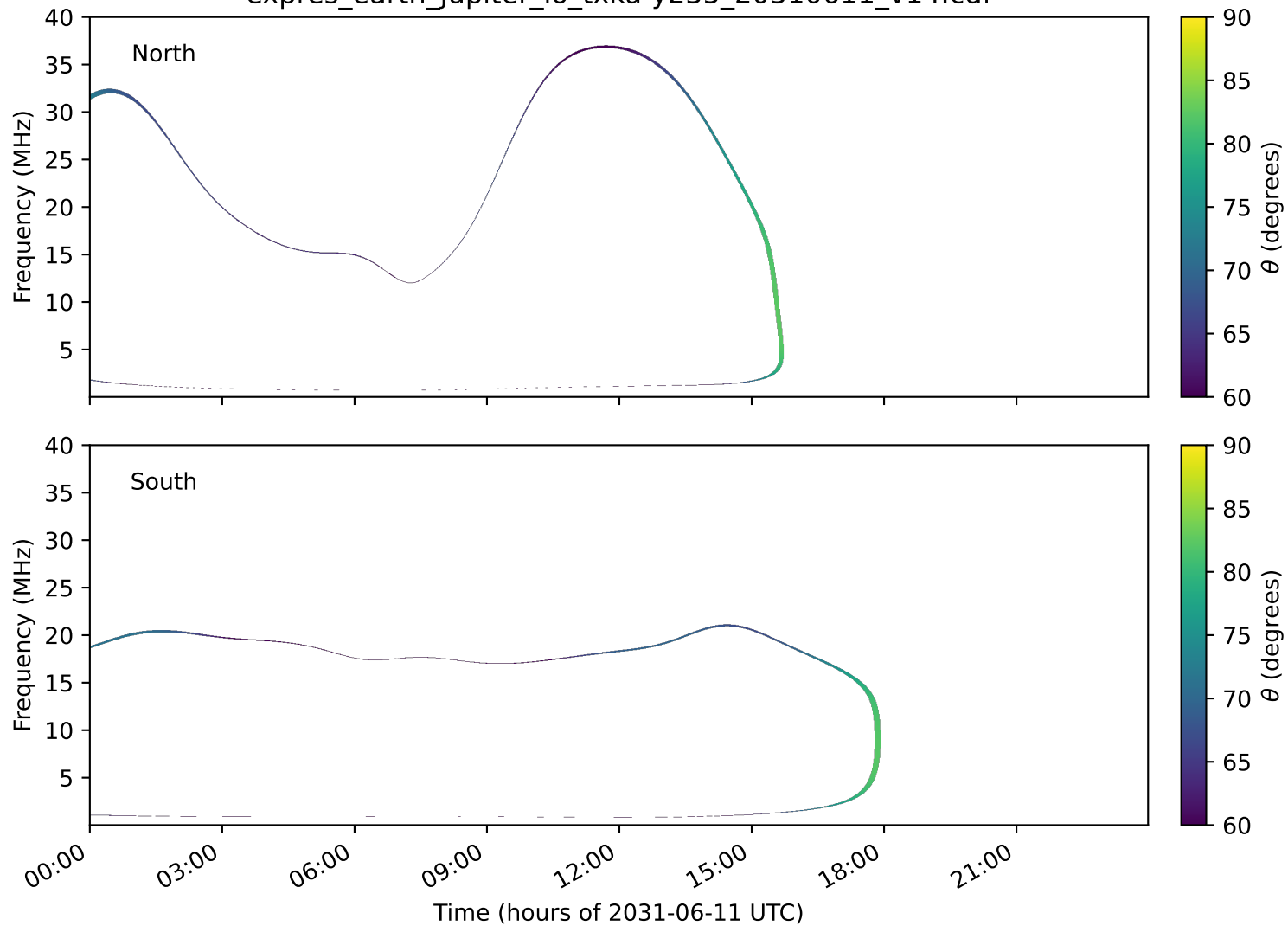
expres_earth_jupiter_io_txka-y235_20310611_v14.cdf
