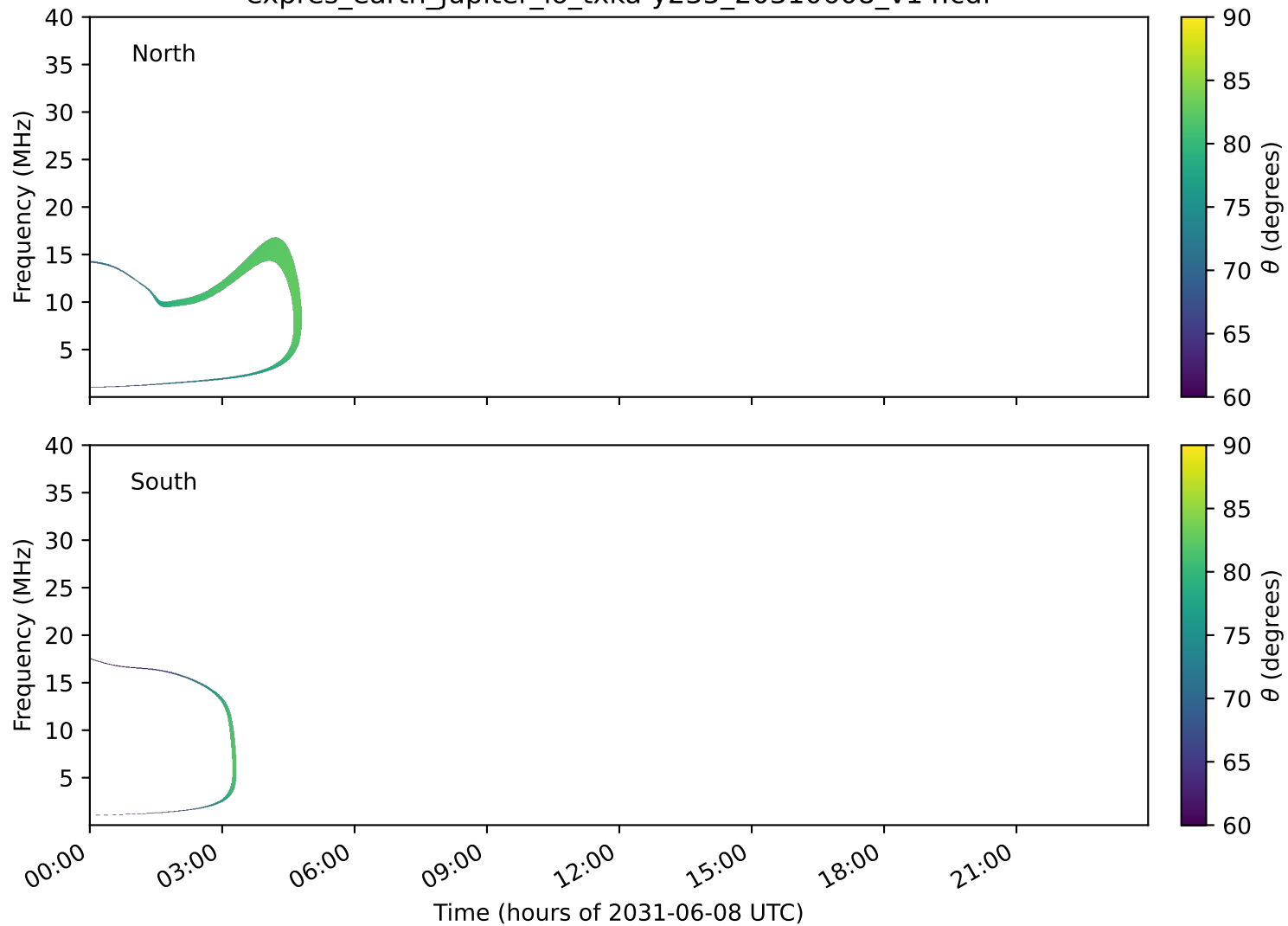
expres_earth_jupiter_io_txka-y235_20310608_v14.cdf
