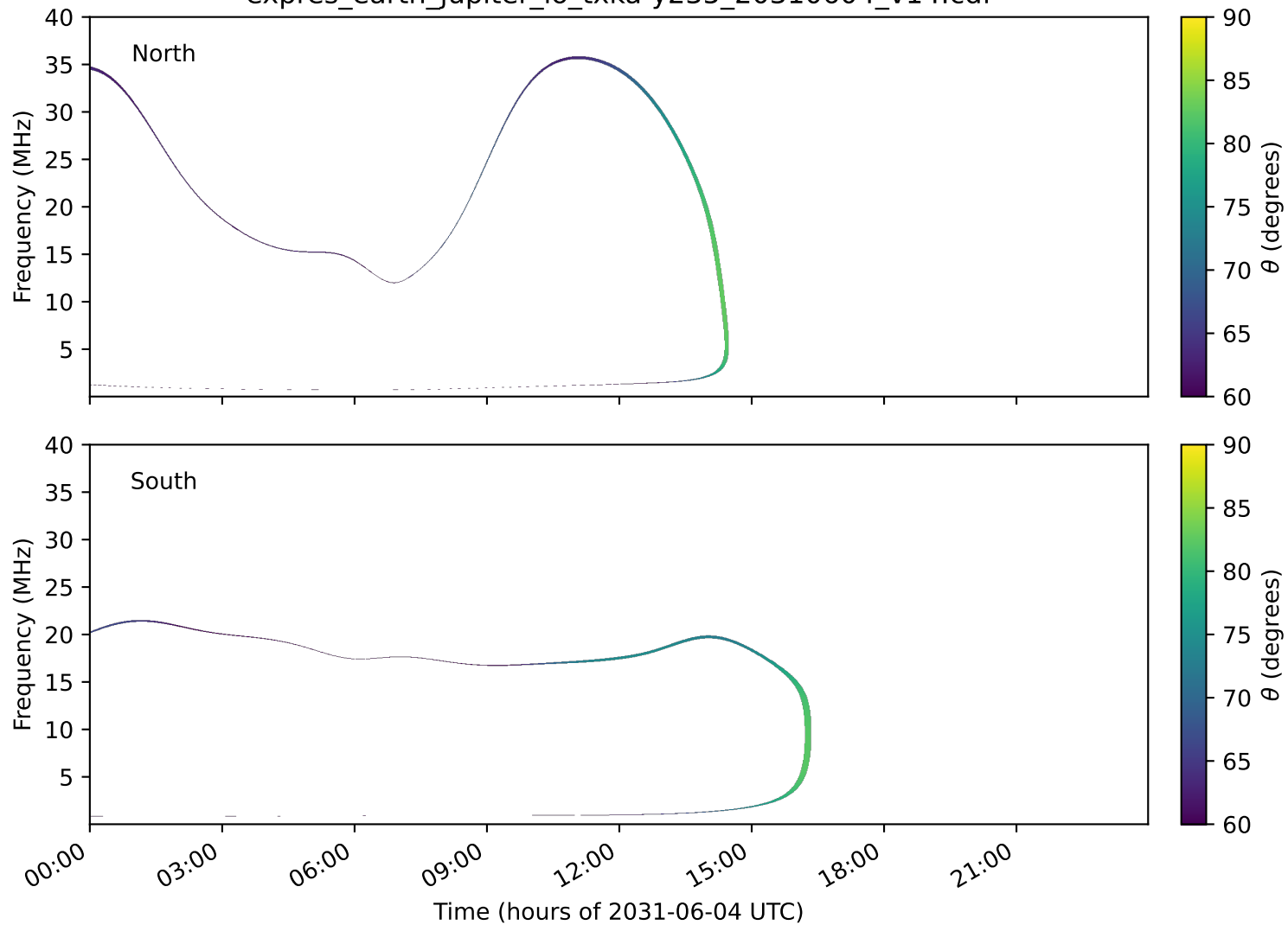
expres_earth_jupiter_io_txka-y235_20310604_v14.cdf
