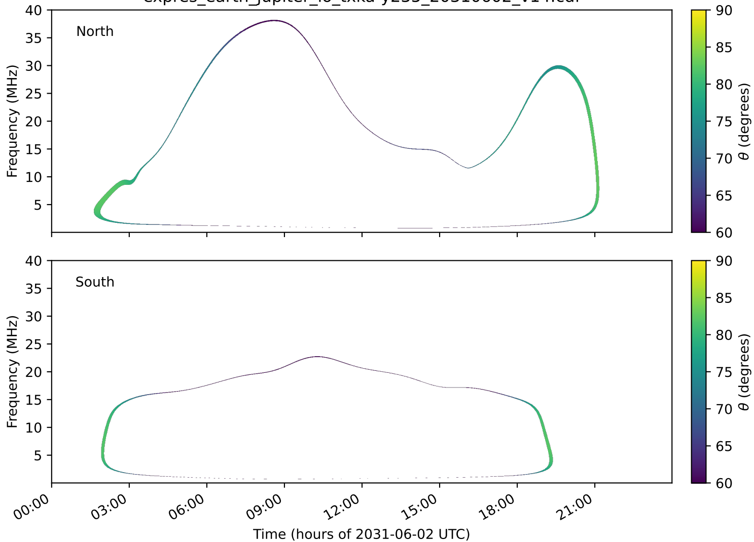
expres_earth_jupiter_io_txka-y235_20310602_v14.cdf
