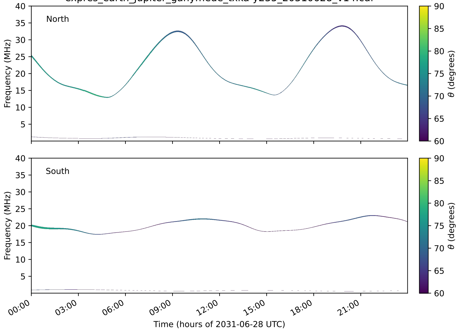
expres_earth_jupiter_ganymede_txka-y235_20310628_v14.cdf
