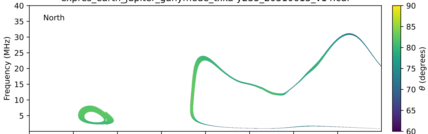
expres_earth_jupiter_ganymede_txka-y235_20310613_v14.cdf
