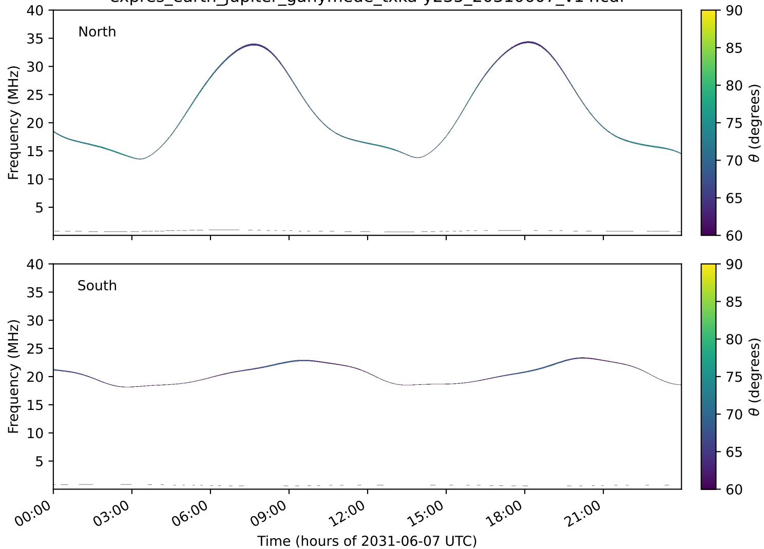
expres_earth_jupiter_ganymede_txka-y235_20310607_v14.cdf
