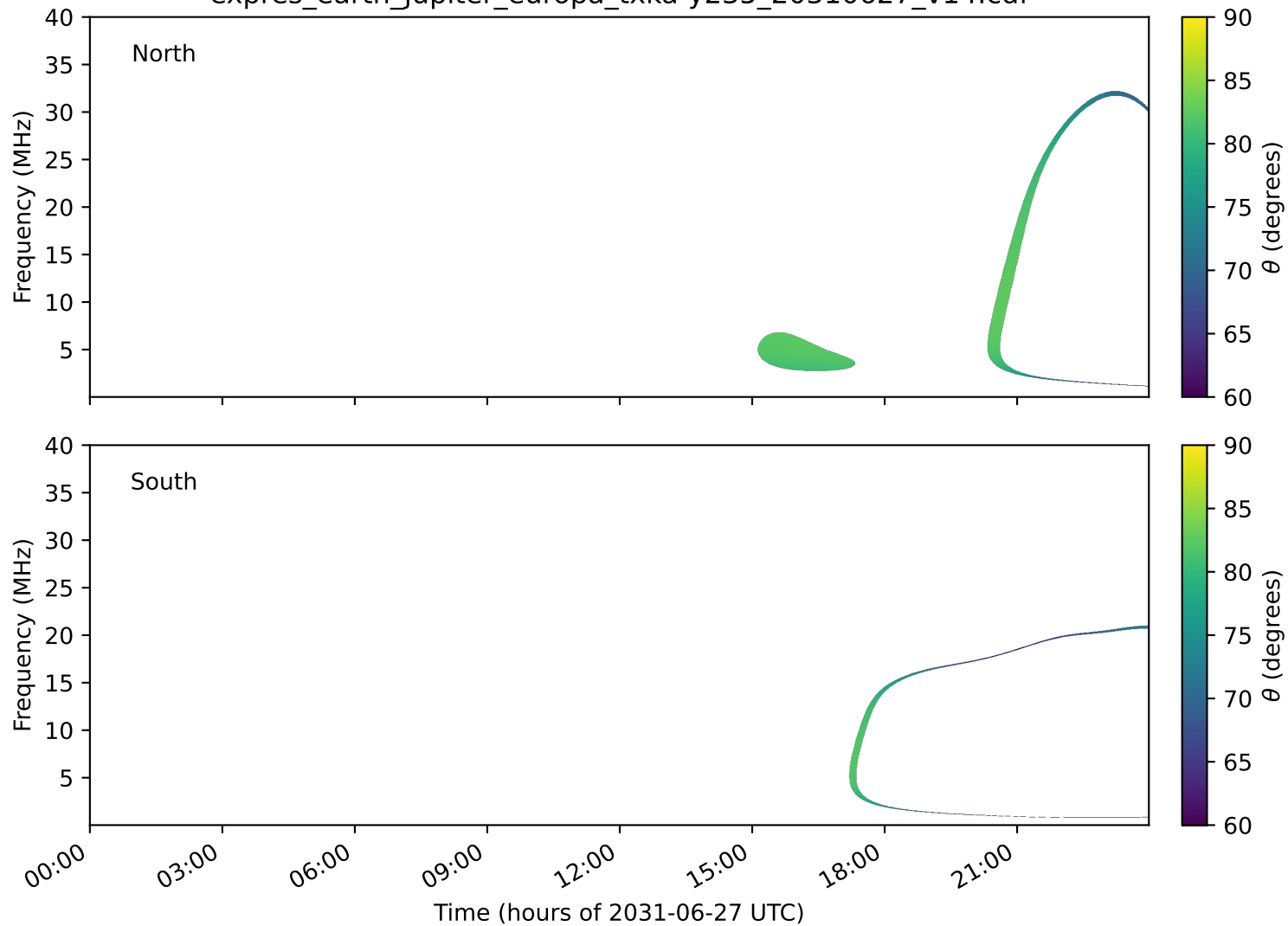
expres_earth_jupiter_europa_txka-y235_20310627_v14.cdf
