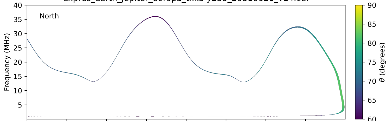
expres_earth_jupiter_europa_txka-y235_20310621_v14.cdf
