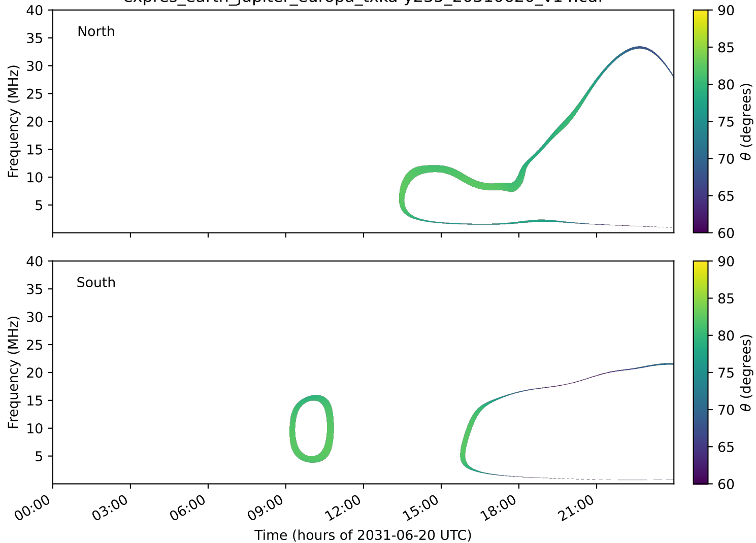
expres_earth_jupiter_europa_txka-y235_20310620_v14.cdf
