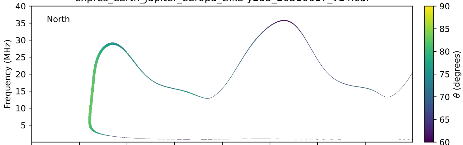
expres_earth_jupiter_europa_txka-y235_20310617_v14.cdf
