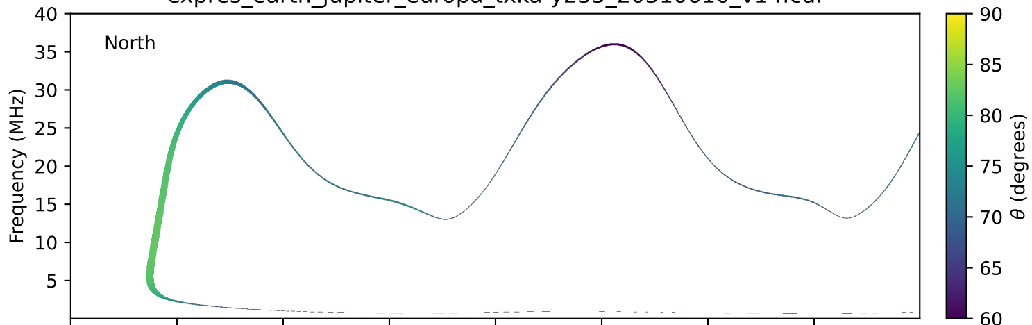
expres_earth_jupiter_europa_txka-y235_20310610_v14.cdf
