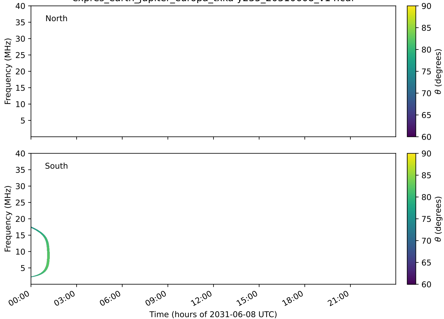
expres_earth_jupiter_europa_txka-y235_20310608_v14.cdf
