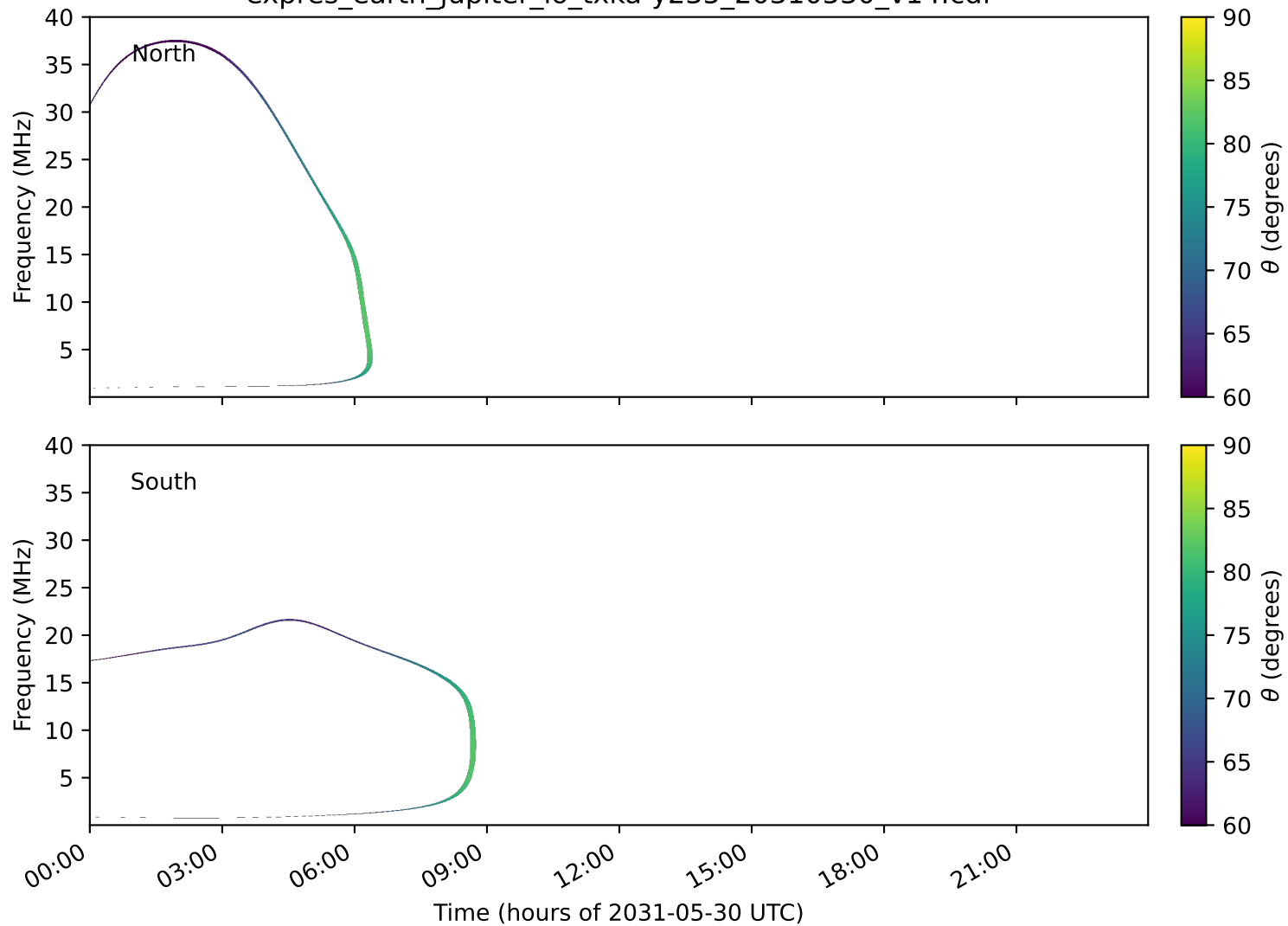
expres_earth_jupiter_io_txka-y235_20310530_v14.cdf
