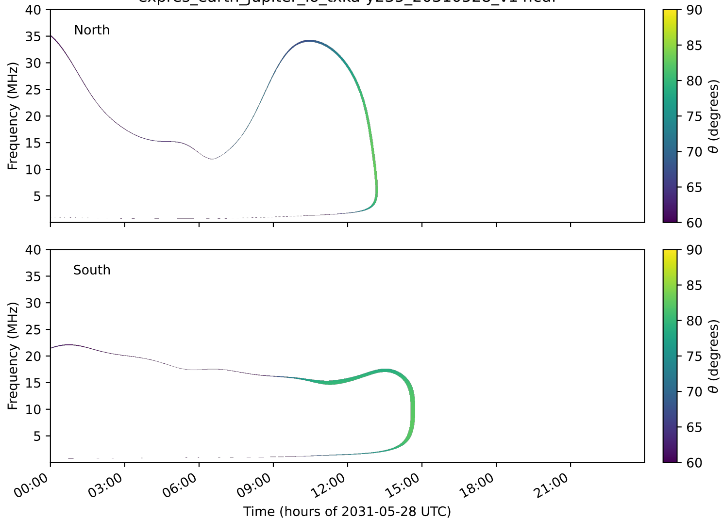
expres_earth_jupiter_io_txka-y235_20310528_v14.cdf
