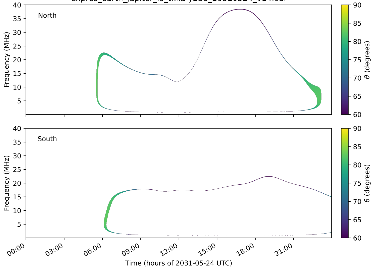
expres_earth_jupiter_io_txka-y235_20310524_v14.cdf
