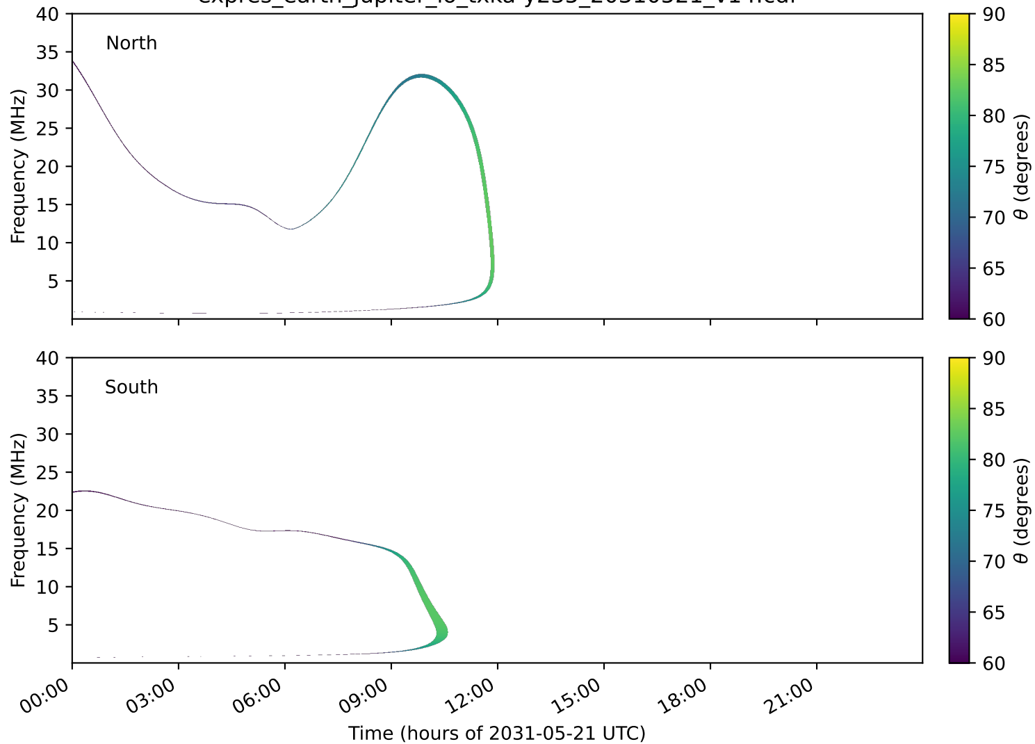
expres_earth_jupiter_io_txka-y235_20310521_v14.cdf
