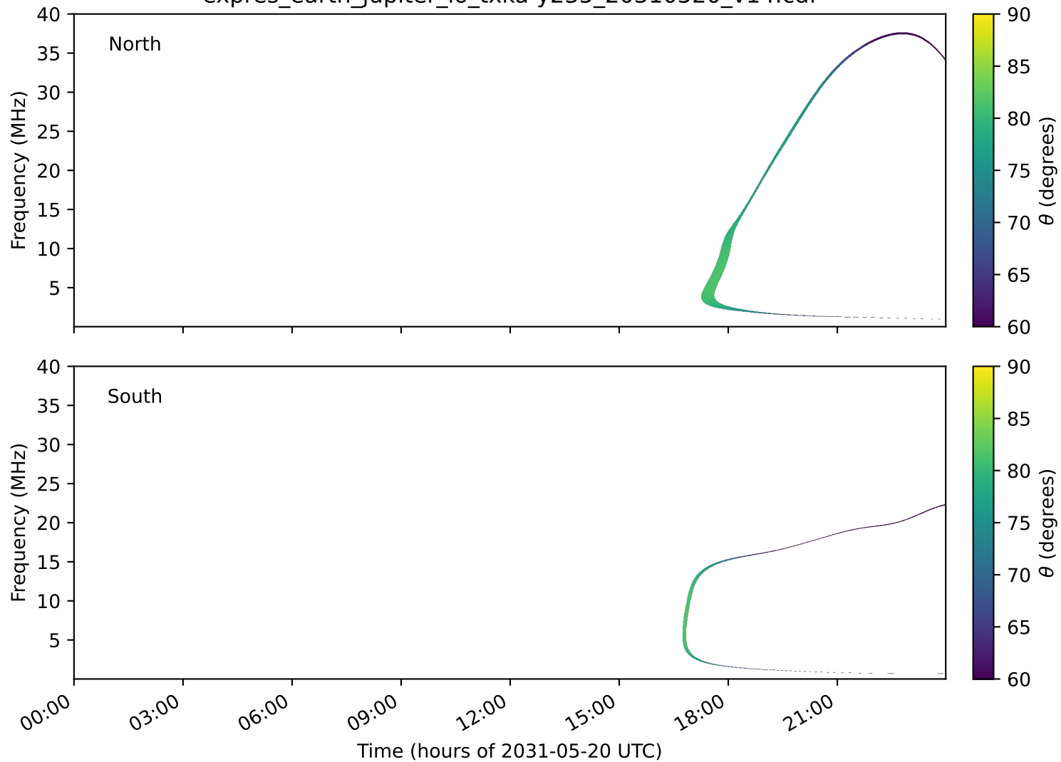
expres_earth_jupiter_io_txka-y235_20310520_v14.cdf
