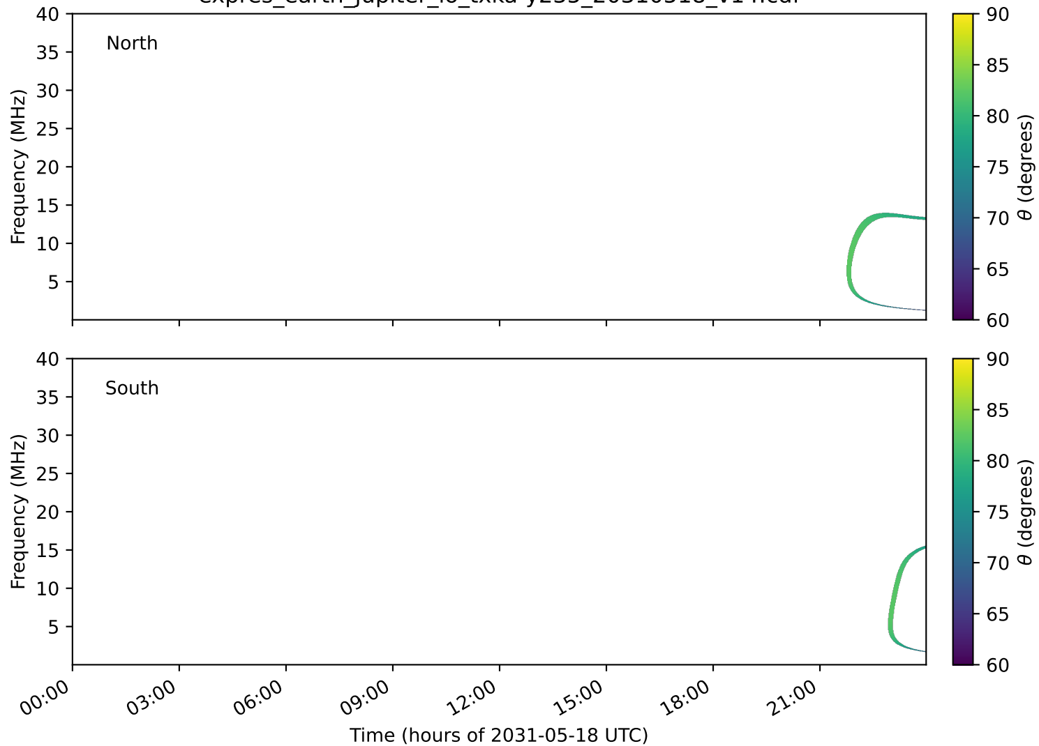
expres_earth_jupiter_io_txka-y235_20310518_v14.cdf
