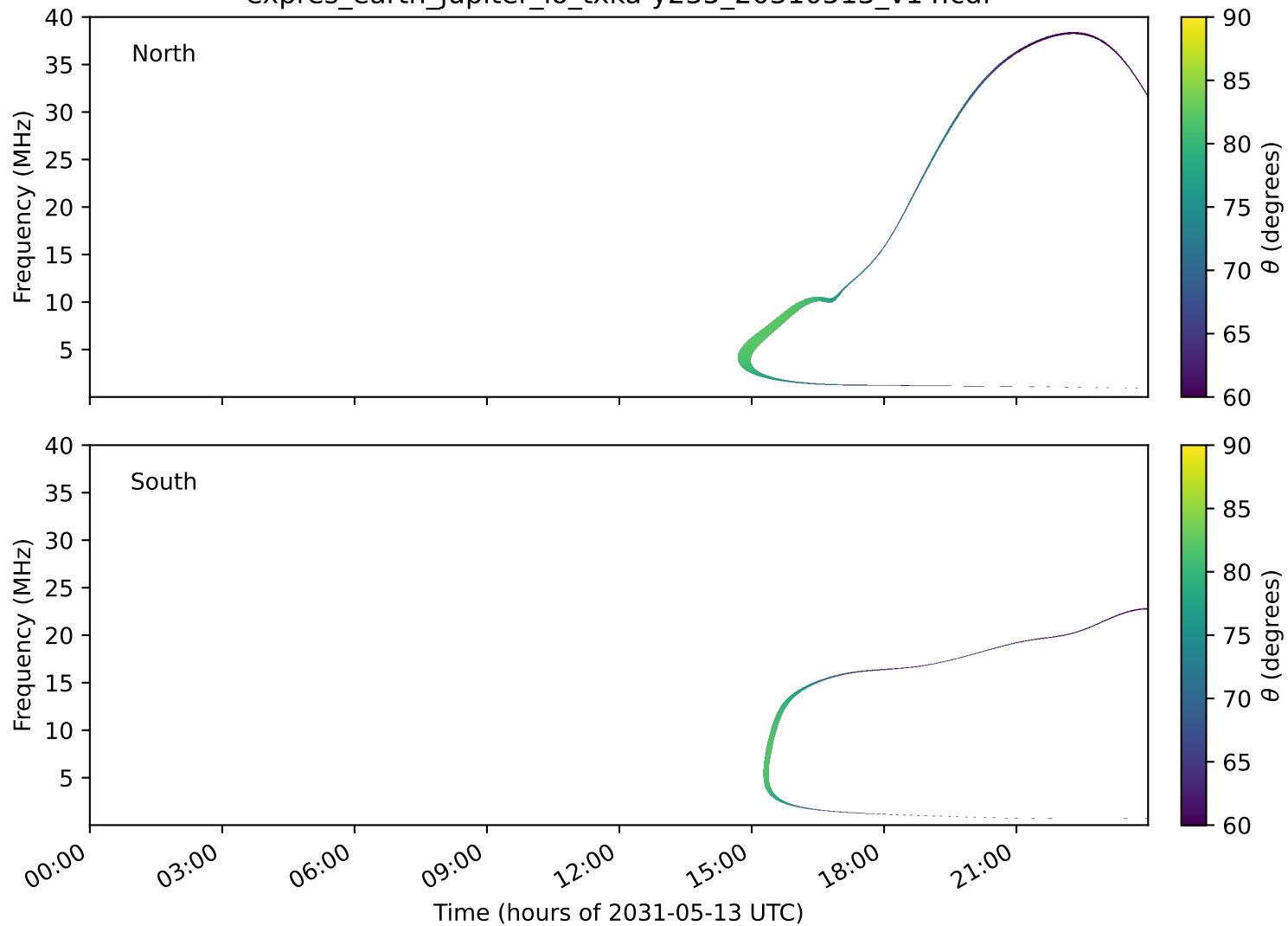
expres_earth_jupiter_io_txka-y235_20310513_v14.cdf
