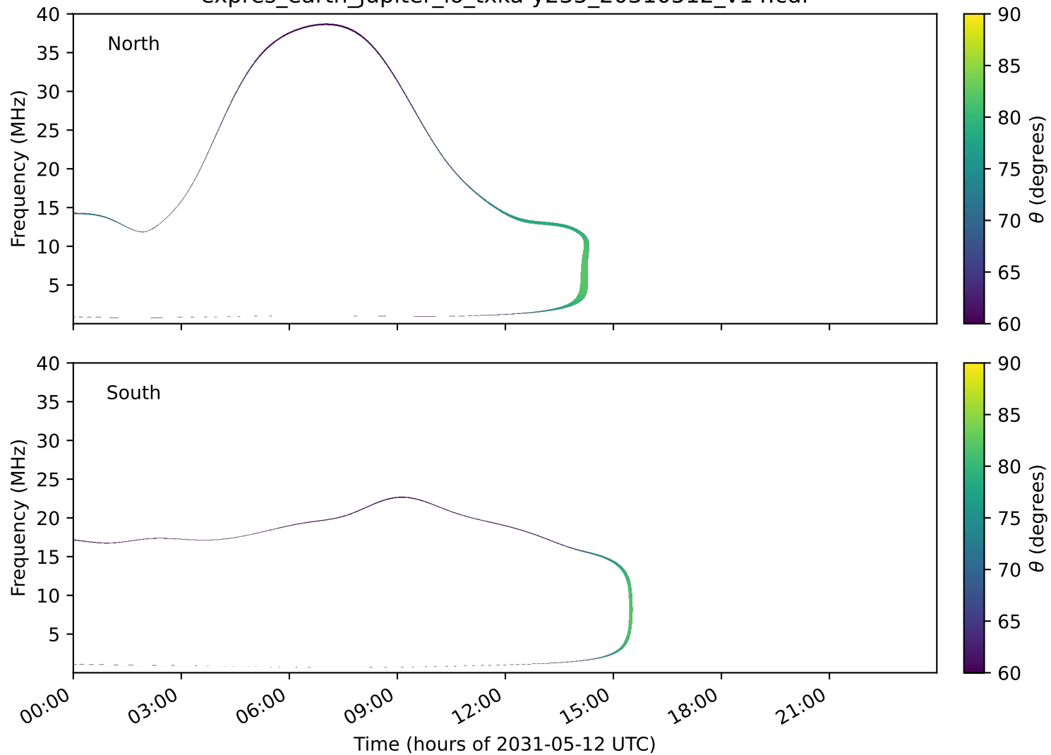
expres_earth_jupiter_io_txka-y235_20310512_v14.cdf
