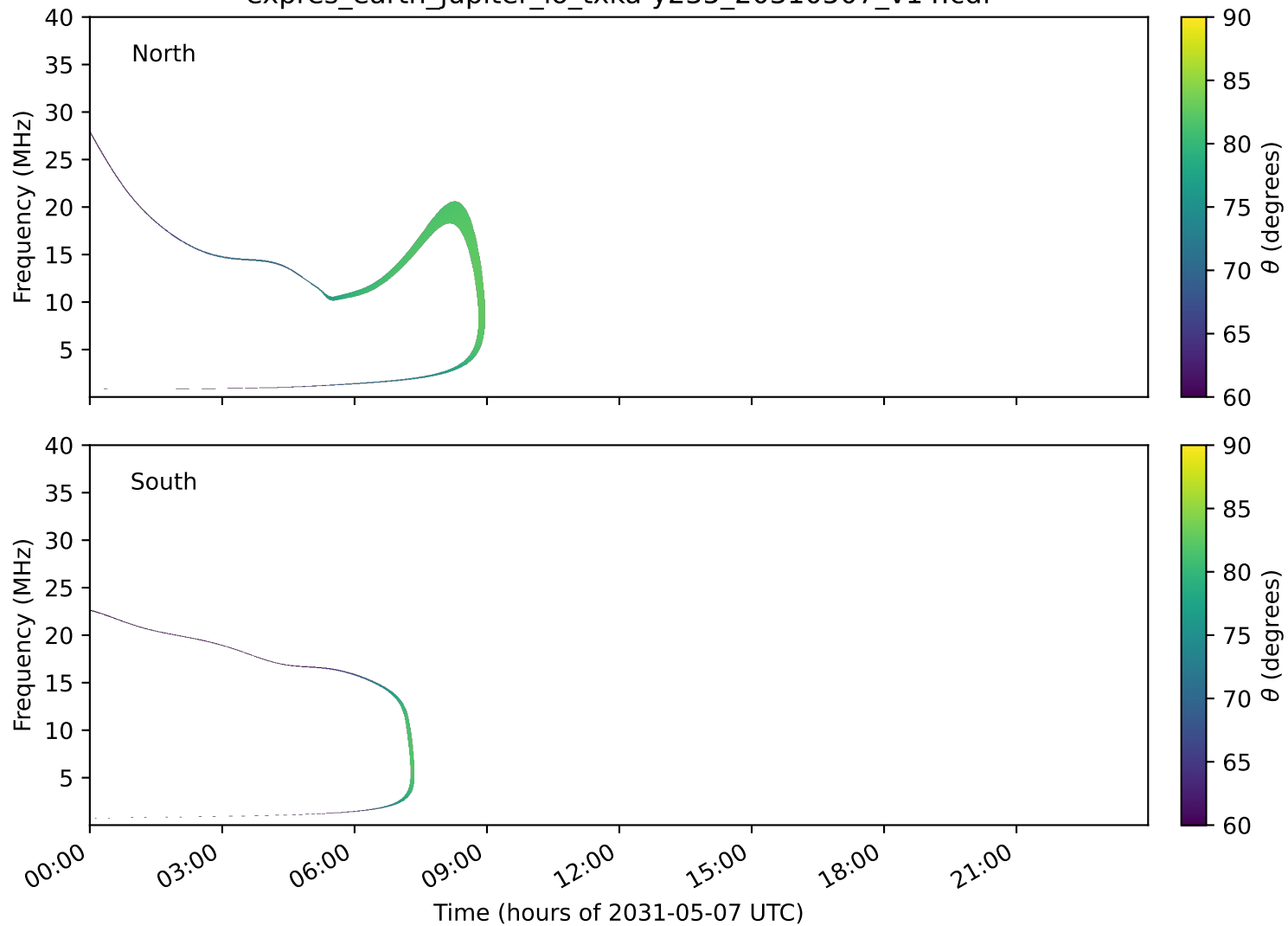
expres_earth_jupiter_io_txka-y235_20310507_v14.cdf
