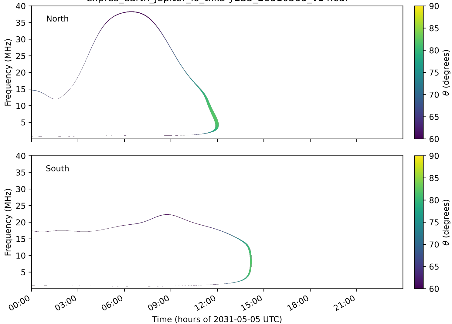
expres_earth_jupiter_io_txka-y235_20310505_v14.cdf
