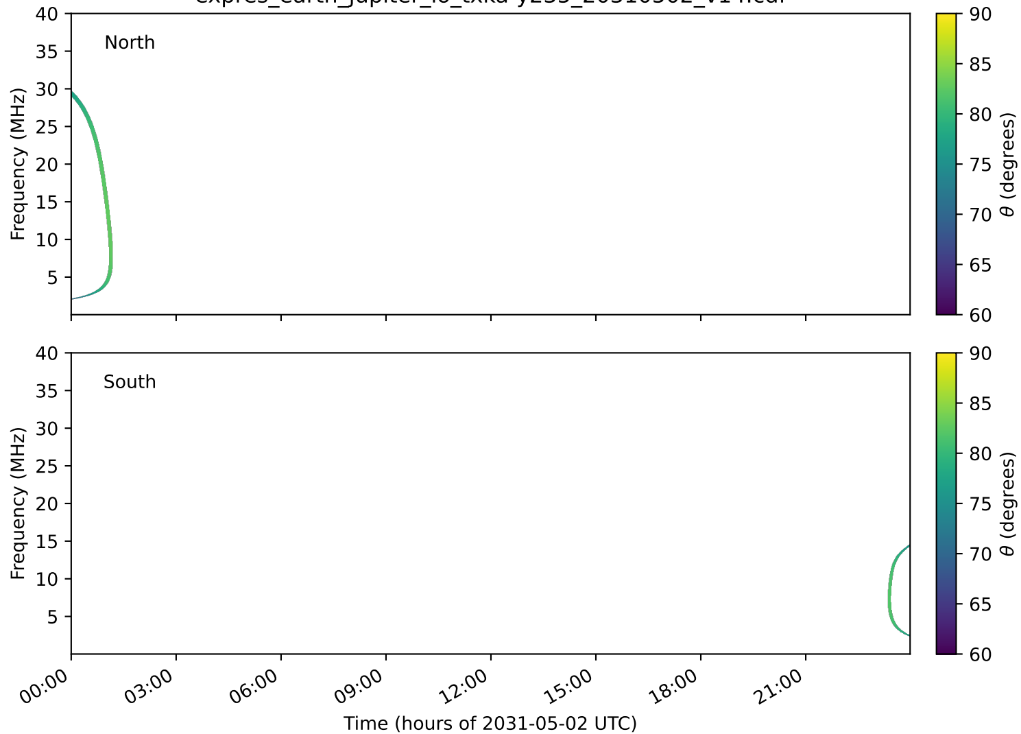
expres_earth_jupiter_io_txka-y235_20310502_v14.cdf
