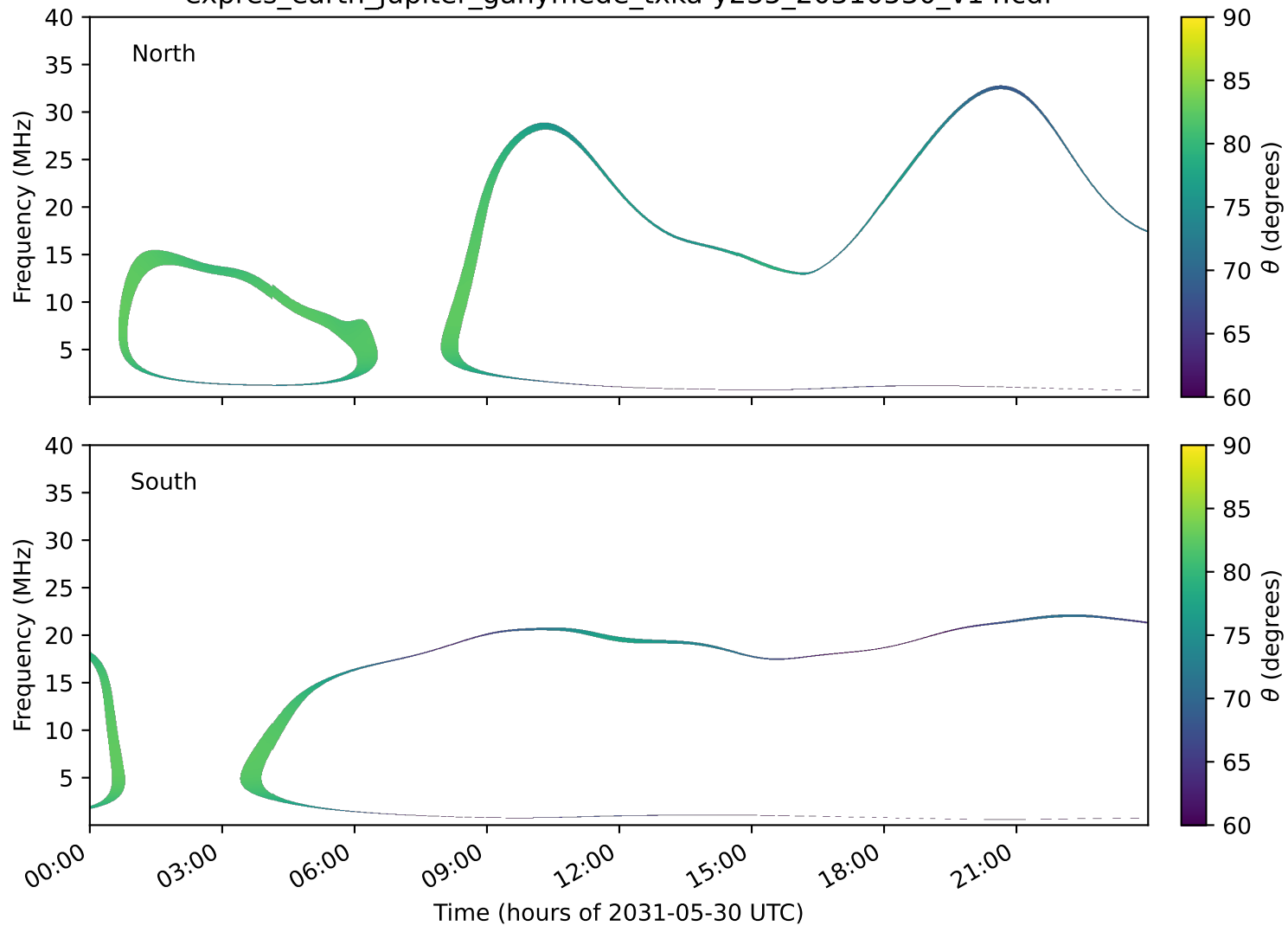
expres_earth_jupiter_ganymede_txka-y235_20310530_v14.cdf
