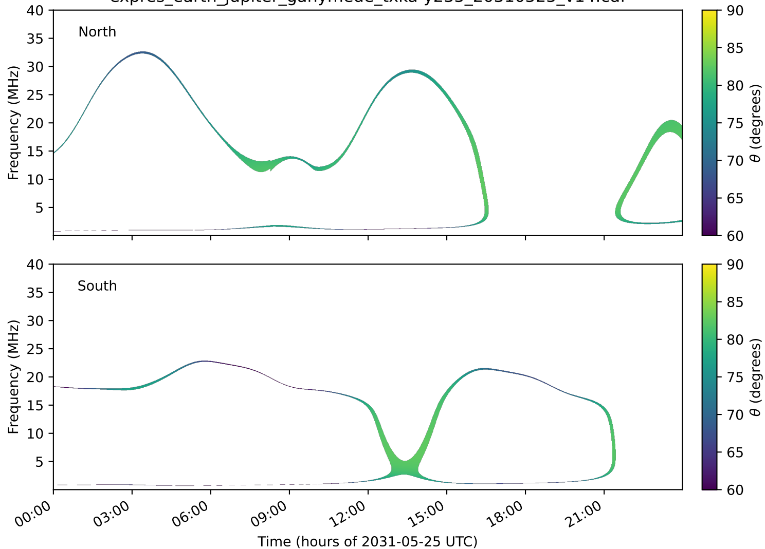
expres_earth_jupiter_ganymede_txka-y235_20310525_v14.cdf
