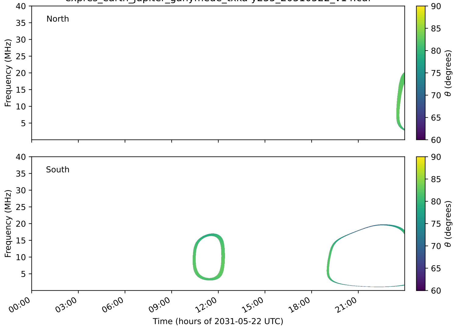
expres_earth_jupiter_ganymede_txka-y235_20310522_v14.cdf
