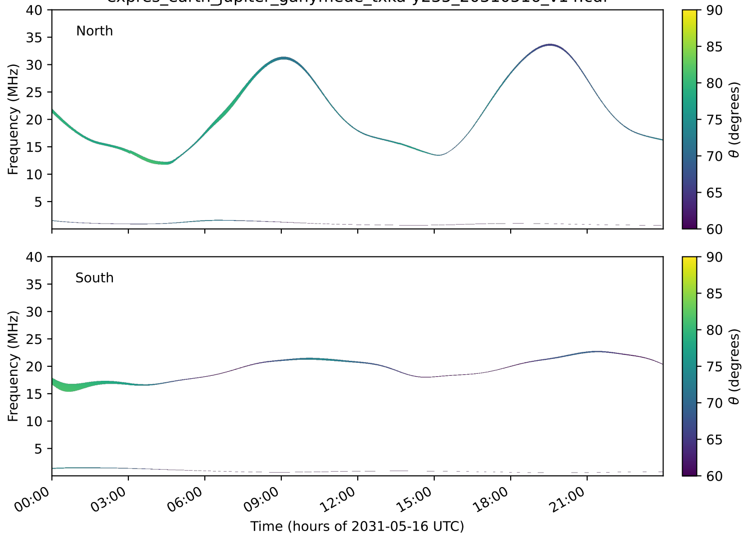
expres_earth_jupiter_ganymede_txka-y235_20310516_v14.cdf
