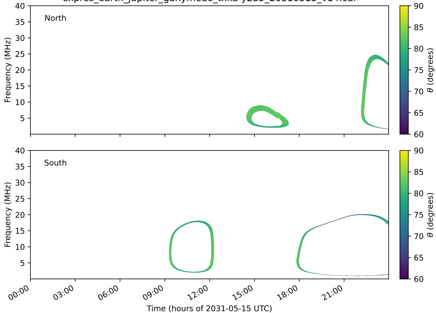
expres_earth_jupiter_ganymede_txka-y235_20310515_v14.cdf
