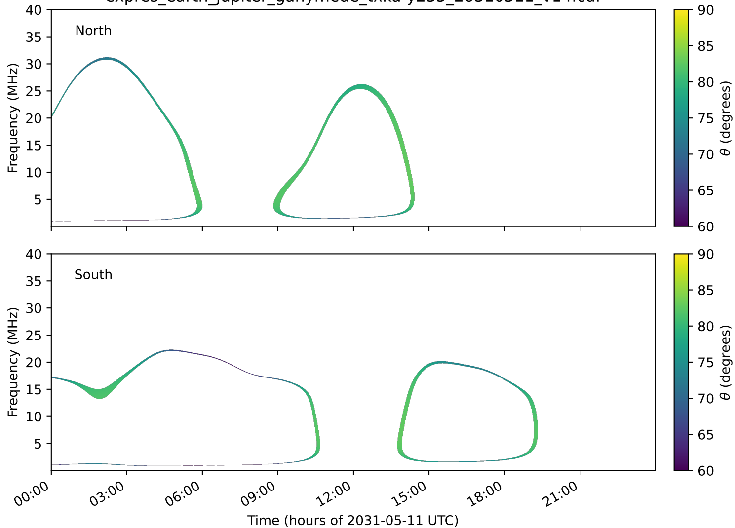
expres_earth_jupiter_ganymede_txka-y235_20310511_v14.cdf
