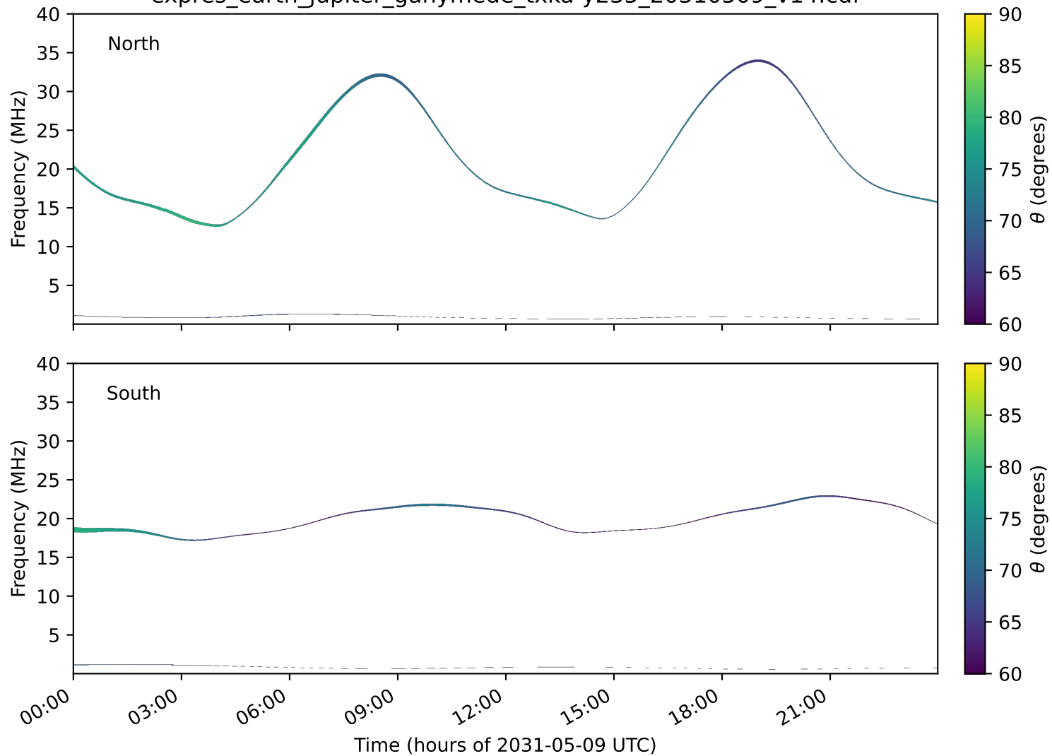
expres_earth_jupiter_ganymede_txka-y235_20310509_v14.cdf
