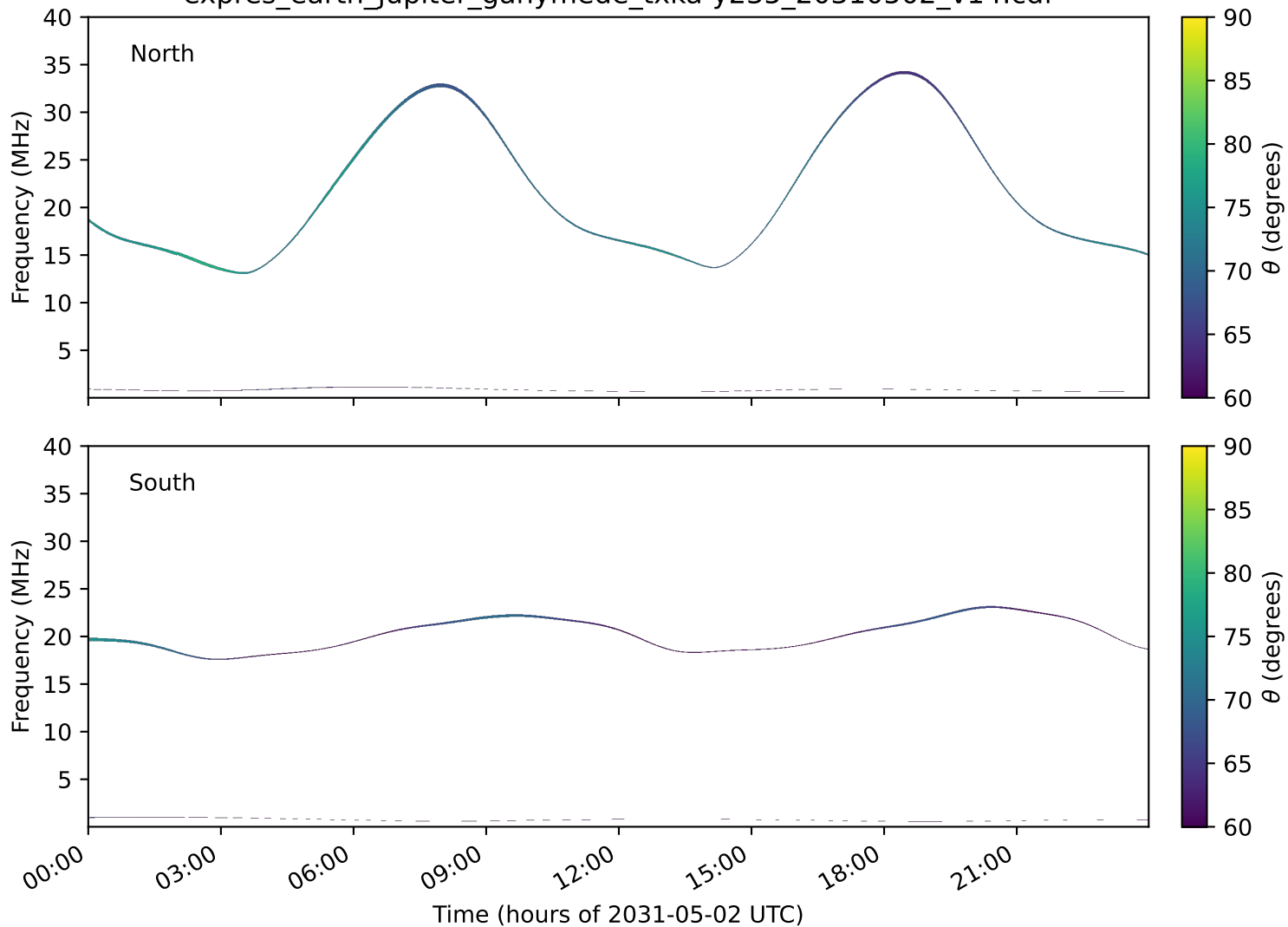
expres_earth_jupiter_ganymede_txka-y235_20310502_v14.cdf
