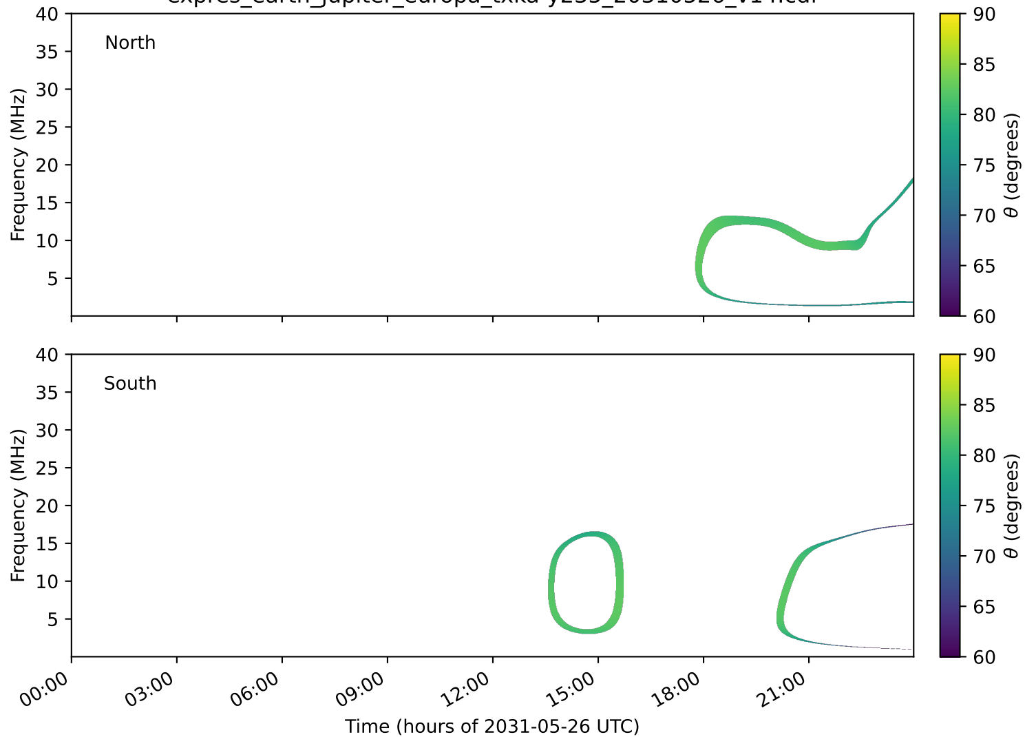
expres_earth_jupiter_europa_txka-y235_20310526_v14.cdf
