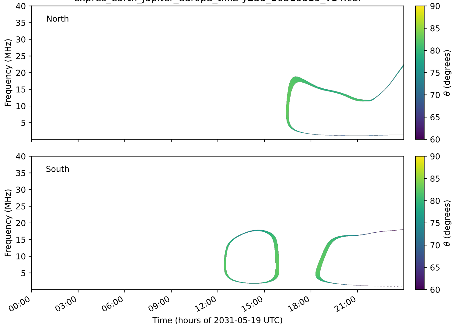
expres_earth_jupiter_europa_txka-y235_20310519_v14.cdf
