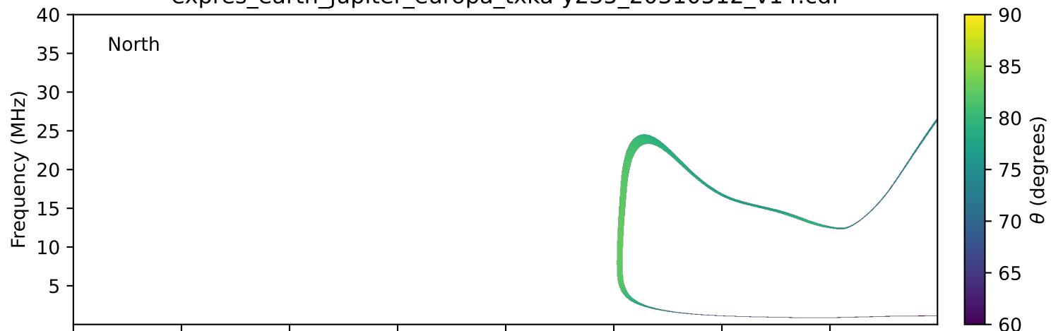
expres_earth_jupiter_europa_txka-y235_20310512_v14.cdf
