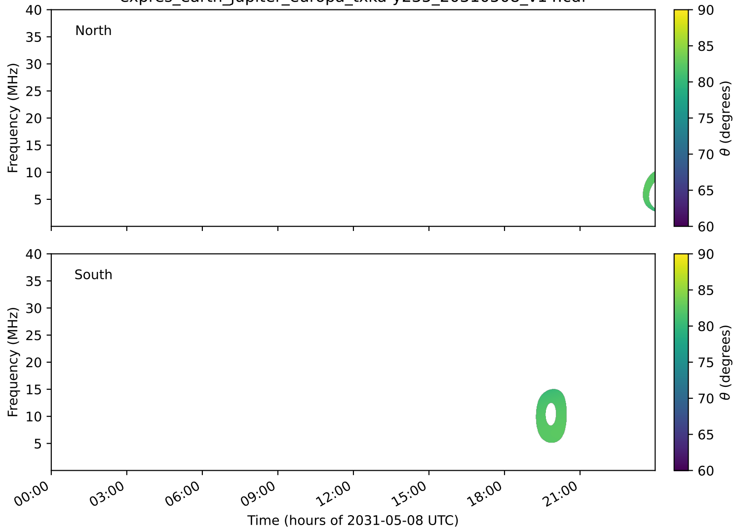
expres_earth_jupiter_europa_txka-y235_20310508_v14.cdf
