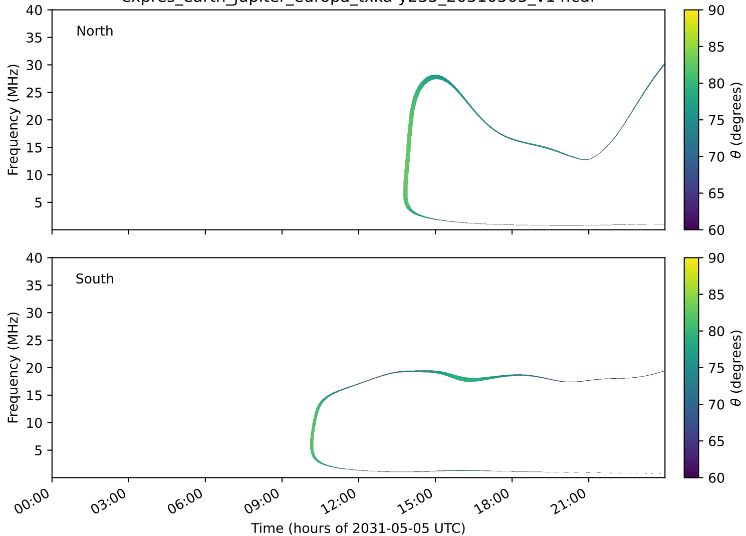
expres_earth_jupiter_europa_txka-y235_20310505_v14.cdf
