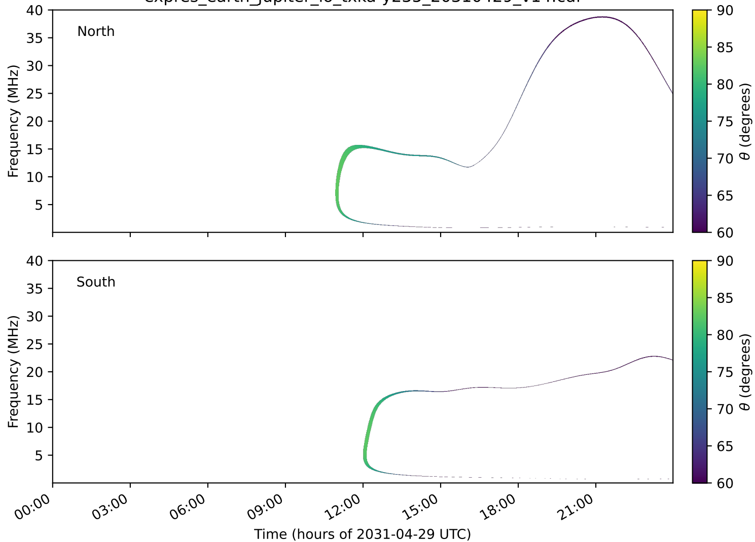
expres_earth_jupiter_io_txka-y235_20310429_v14.cdf
