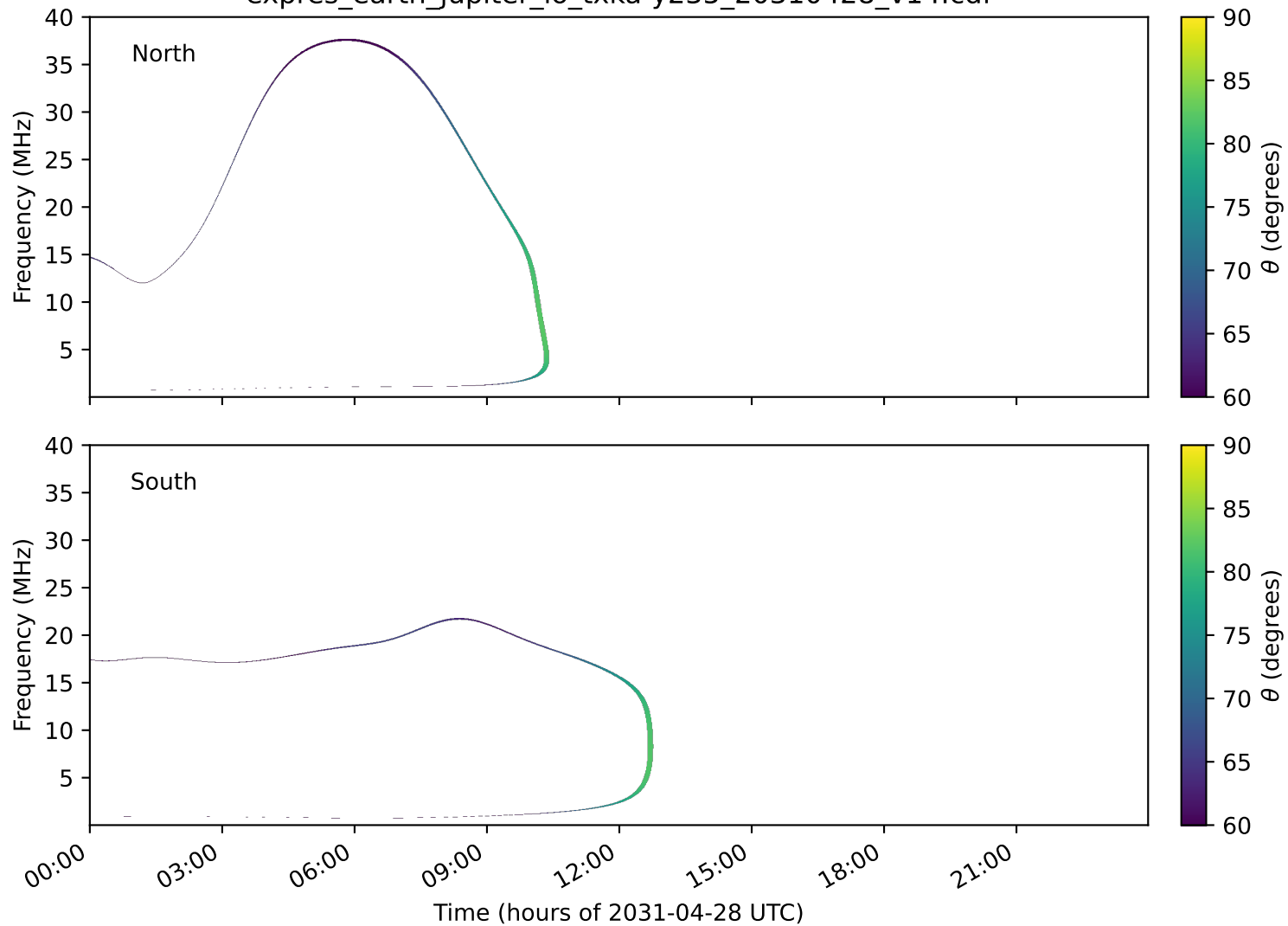
expres_earth_jupiter_io_txka-y235_20310428_v14.cdf
