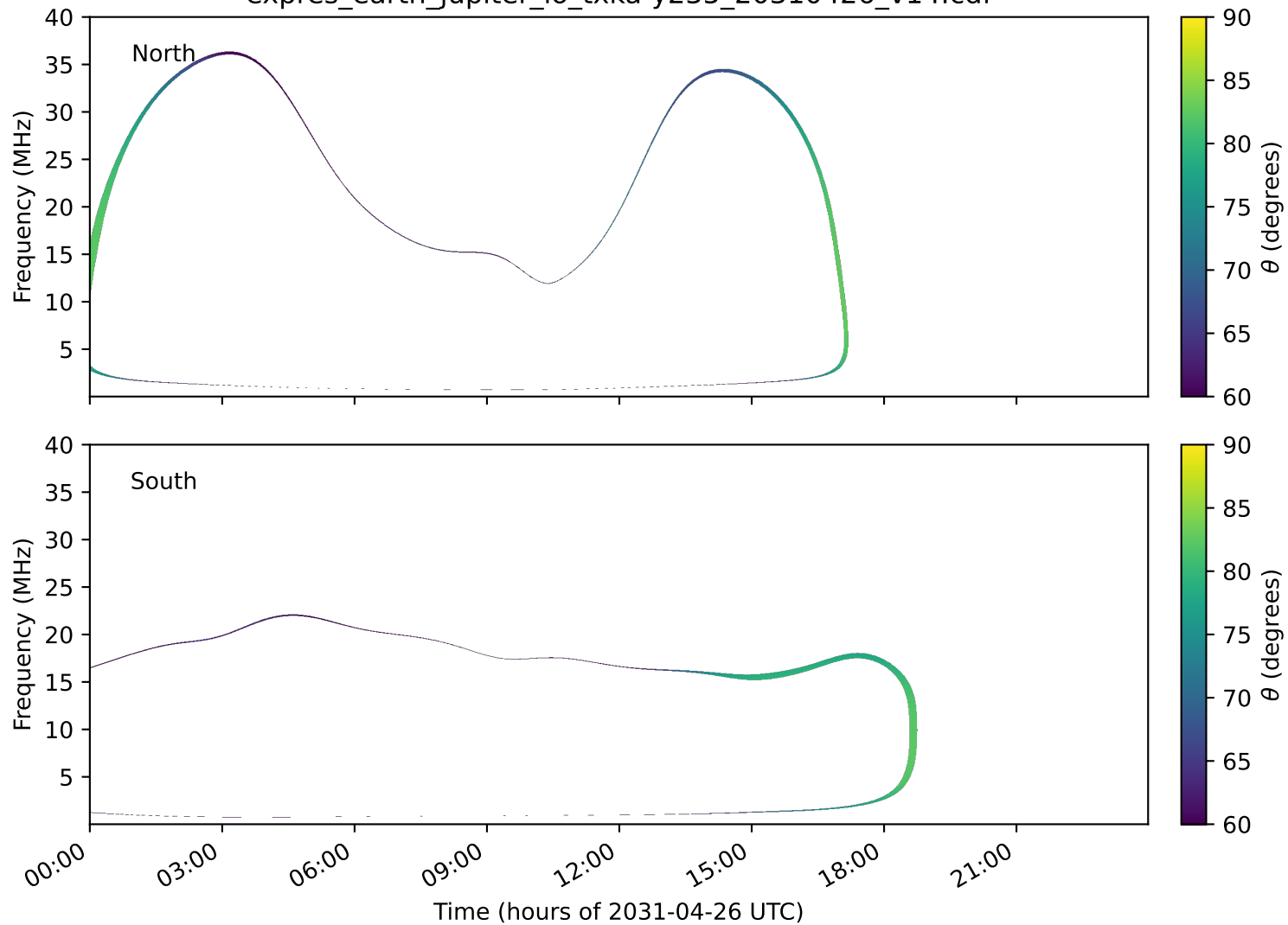
expres_earth_jupiter_io_txka-y235_20310426_v14.cdf
