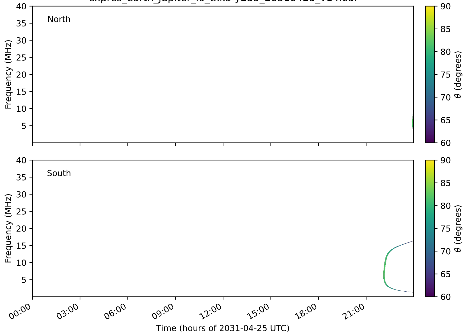
expres_earth_jupiter_io_txka-y235_20310425_v14.cdf
