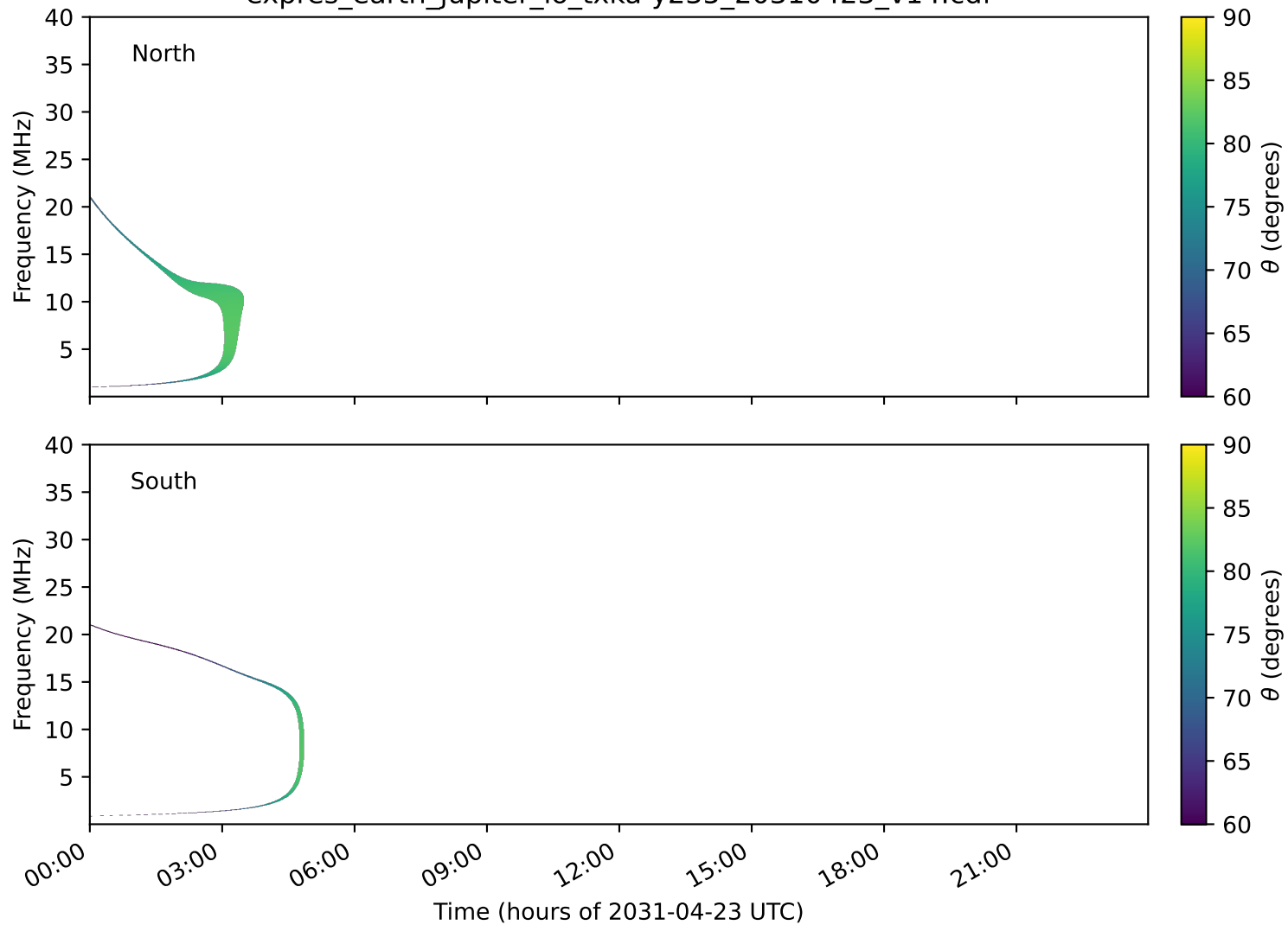
expres_earth_jupiter_io_txka-y235_20310423_v14.cdf
