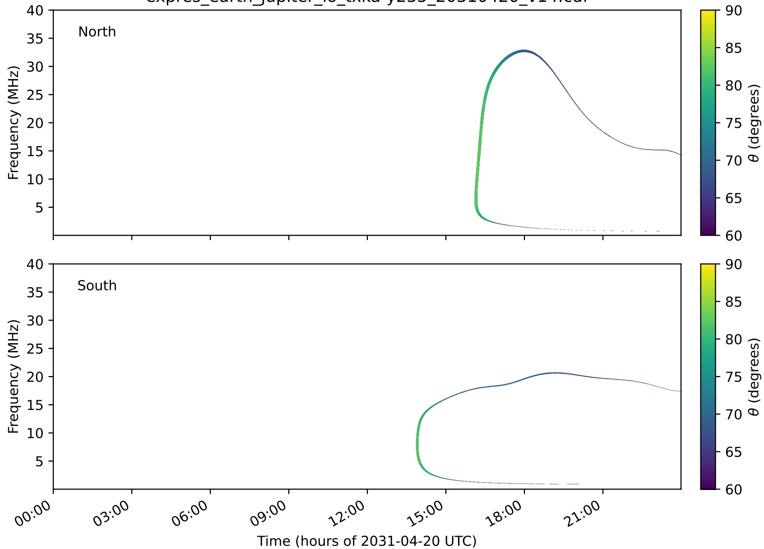
expres_earth_jupiter_io_txka-y235_20310420_v14.cdf
