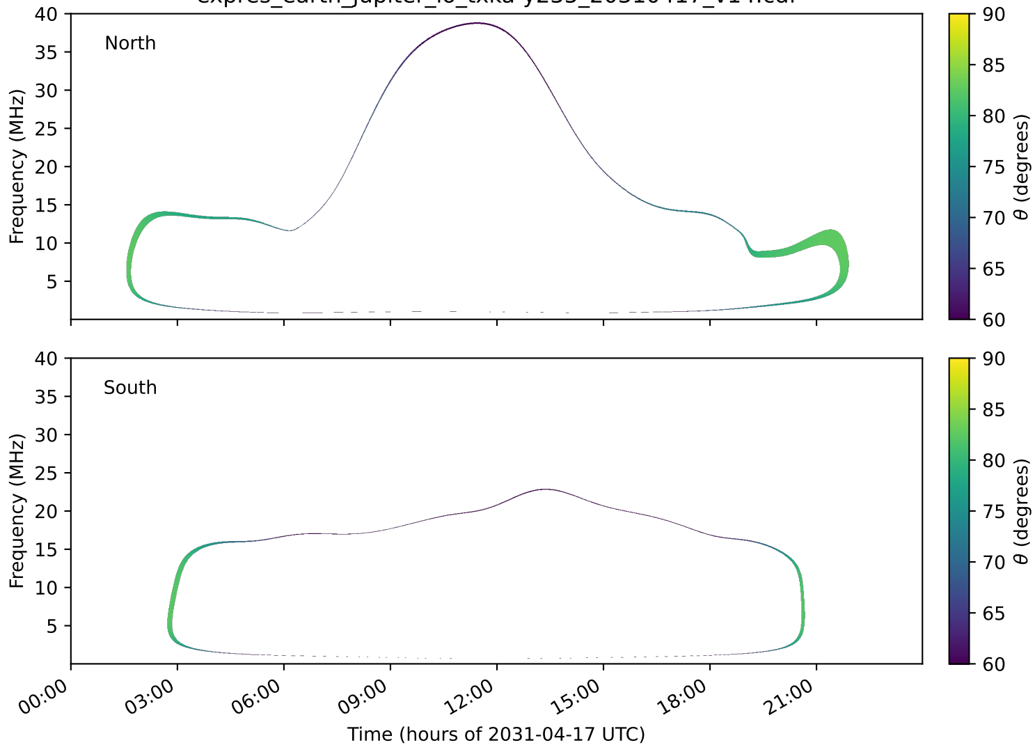
expres_earth_jupiter_io_txka-y235_20310417_v14.cdf
